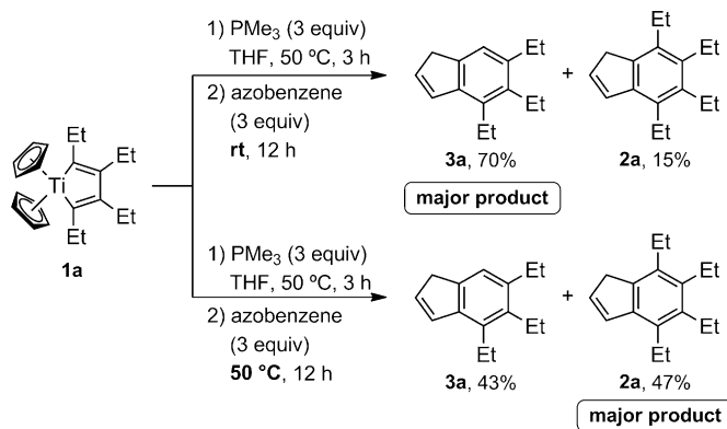
Scheme 10. Formation of indene derivatives with \text{PMe}_3 and azobenzene at various temperatures.
