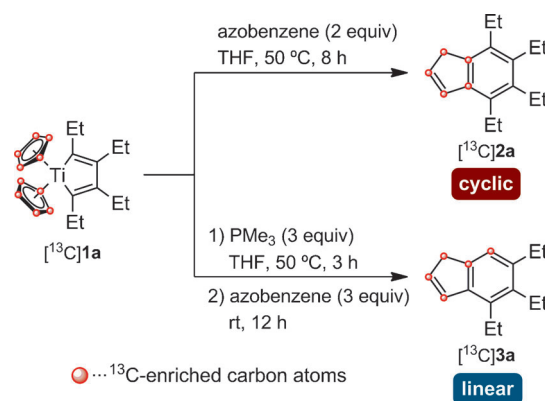
Scheme 4. 13 C-Labeling experiment for the formation of indenenes 2a and 3a .
